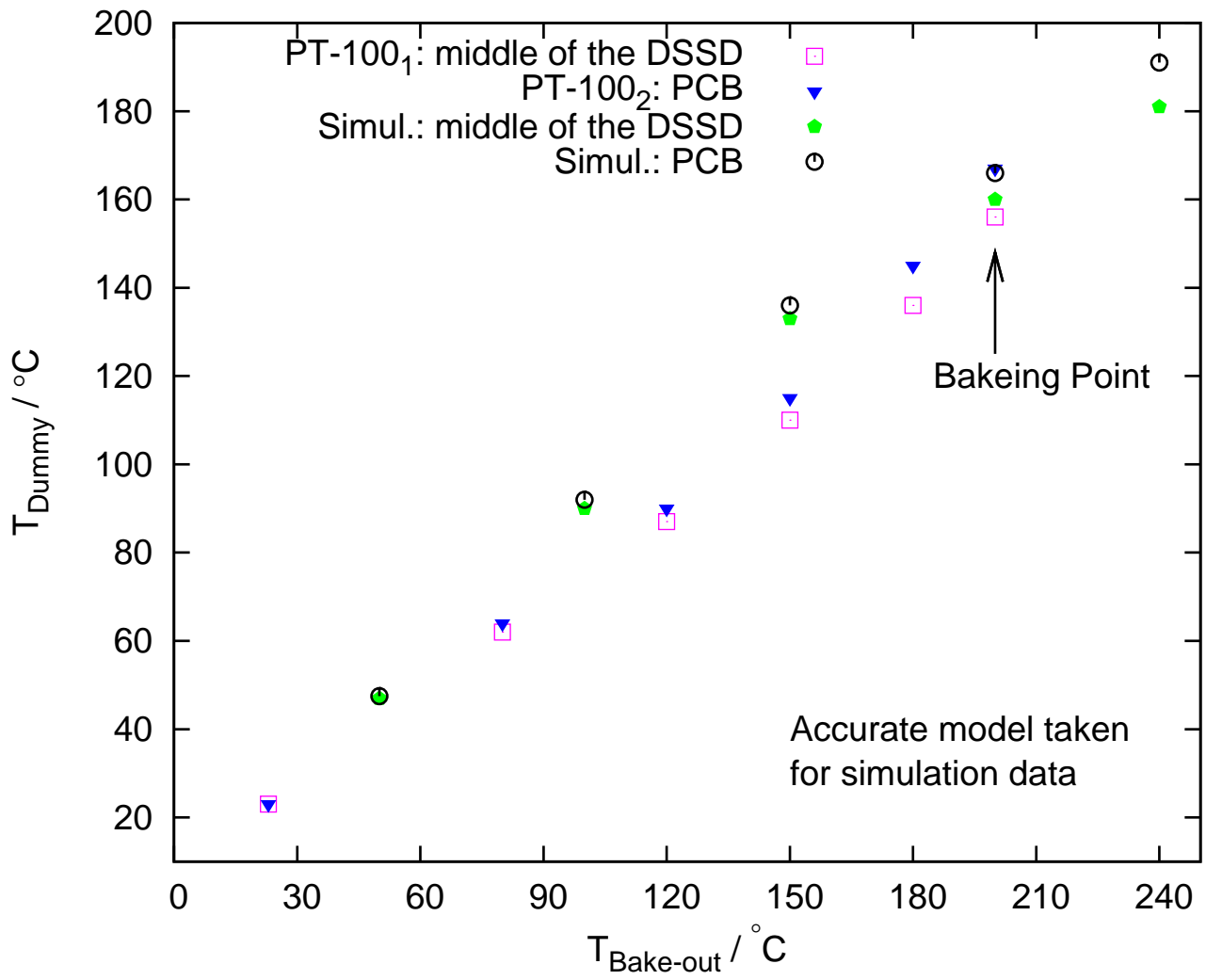
Temperature Measurement vs. Temperature Simulation
